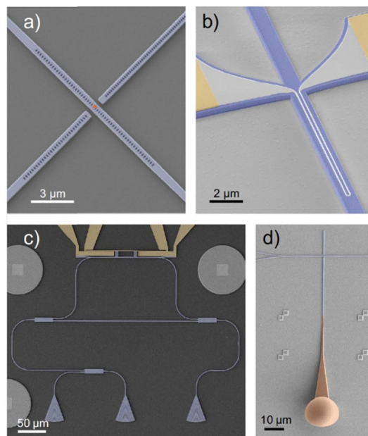
Figure 11. Nanophotonic circuit components for Ta 2 O 5 -on-insulator: (a) nanodiamonds (orange) containing quantum emitters coupled to 1D-photon crystal cavities (blue) in Ta 2 O 5 -waveguides for optical excitation and single-photon collection. (b) Ta 2 O 5 -waveguide-integrated SNSPD (white). (c) Opto-electromechanical phase shifter (top) embedded in a Mach-Zehnder interferometer formed by multimode interference devices (center) accessible from optical fibers via grating couplers (bottom). (d) Total internal reflection coupler (orange) produced in 3D direct laser writing, providing an efficient optical interface to Ta 2 O 5 -waveguides (blue). Panel (b) reprinted with permission from [70] under a Creative Commons Attribution 4.0 International License . Panel (c) reprinted with permission from [71].
